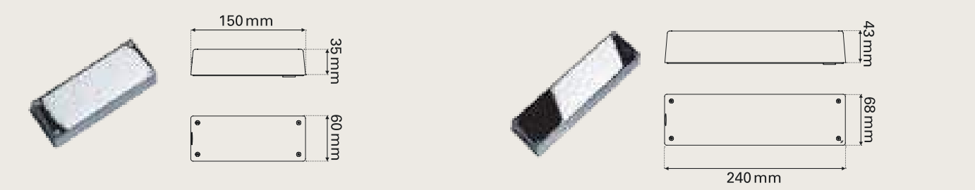
DRIVER BOX S Dimensions : 60 x 35 x 150 mm
